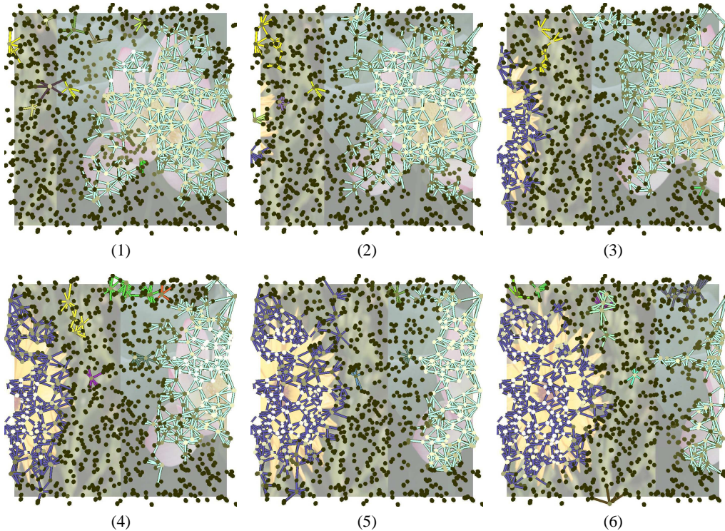
Figure 10: Figure/ground separation over several images from a larger image sequence. Every 100th image is shown. Even though a different set of neurons responds to the visual input, it is still the same connected sub-network as indicated by the color of the sub-network.
