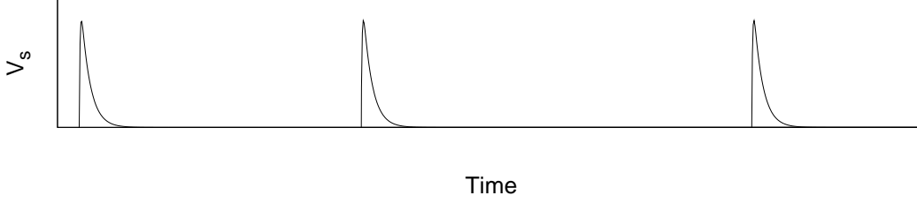
Figure 1: Three spikes traveling along axon.
