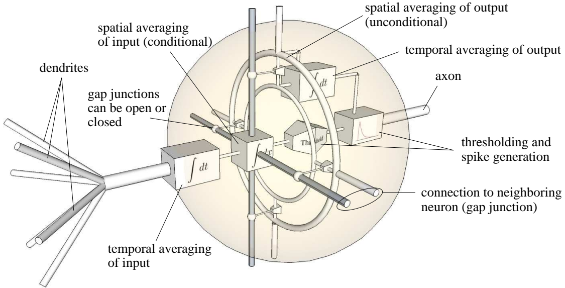
Figure 6: Artificial neuron with lateral connections (gap junctions). The operation of this model is fully specified by the algorithm given in Figure 8.
