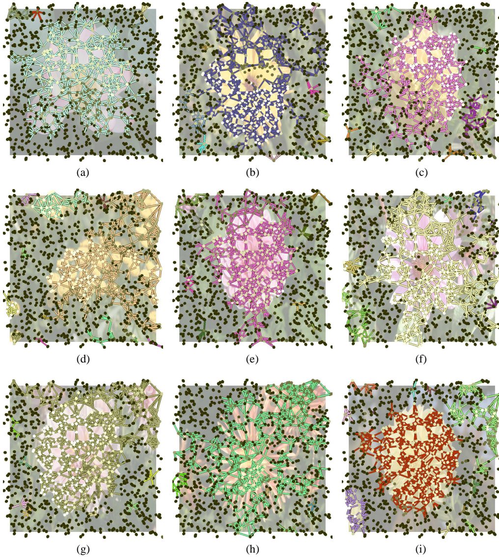
Figure 9: Figure/ground separation using our model. A sheet of neurons (nodes) receives input from a virtual retina (image in background). Gap junctions (connections between nodes) open if the temporal output of a neuron is above the spatial average.
