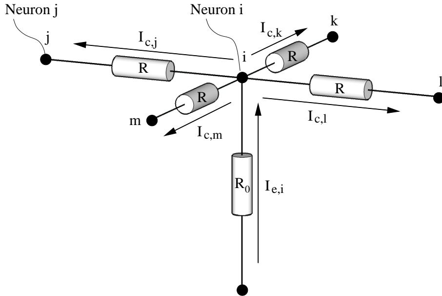
Figure 4: The external current I_{e,i} flowing into node i has to be equivalent to the current exchanged with adjacent nodes.
